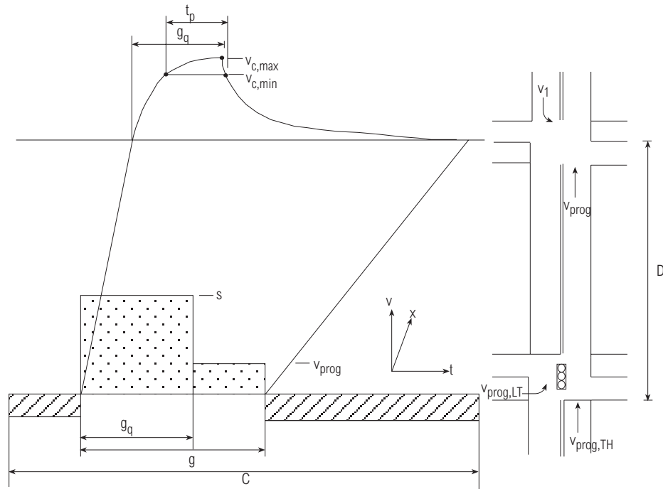
EXHIBIT 17-12. PLATOON DISPERSION MODEL
